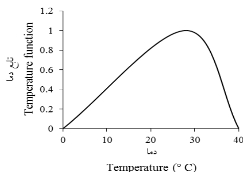
Fig. 2. The beta function for description the development rate to temperature
